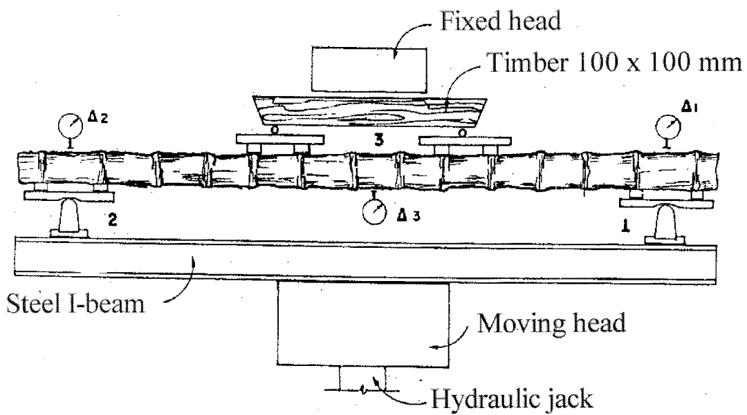
Figure 11 — A bending machine, with an added steel beam (Sotela 1990)
