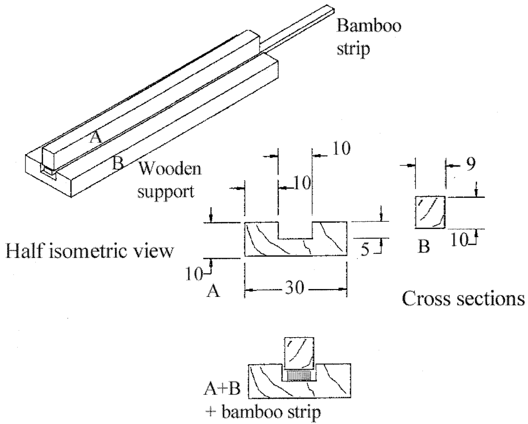
Figure 15 — Tensile test piece with wooden ends
